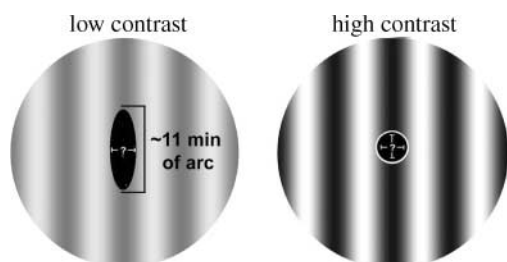
Figure 4. Estimated extent of parallel and orthogonal integration superimposed on a grating like those used as stimuli. The superimposed receptive field illustrates our estimate of 11.0 min of arc of integration along uniform stimulus bars at low contrast, and minimal integration in other conditions. The scale assumes an 8.5 cycles \text{deg}^{-1} carrier.
