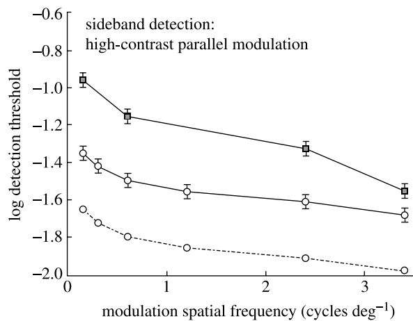
Figure 6. Data for participant T. L. in the sideband-control experiment for the high-contrast, 8.5 \text{ cycles deg}^{-1} carrier condition with parallel modulation. The white circles along the solid line correspond to the thresholds measured for detection of modulation at high contrast and for parallel modulation. Based on these values, we calculated the predicted beat detection thresholds, shown here as white circles along a dotted line. The actual beat thresholds, shown as grey squares, were greater than the prediction, suggesting that sideband detection does not account for modulation detection in the high-contrast case with parallel modulation.
