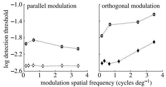
Figure 5. Sideband detection for low contrast: data from participant T. L. in the sideband-control experiment for the low-contrast carrier condition. White circles correspond to detection thresholds for parallel modulation, and black circles to thresholds for orthogonal modulation. The grey squares are the thresholds collected for detection of the lower-frequency sideband corresponding to each modulation direction and spatial frequency. The latter thresholds are higher, suggesting that sideband detection is not governing modulation detection thresholds at low contrast. Here again, carrier spatial frequency is 8.5 cycles \text{deg}^{-1} .
