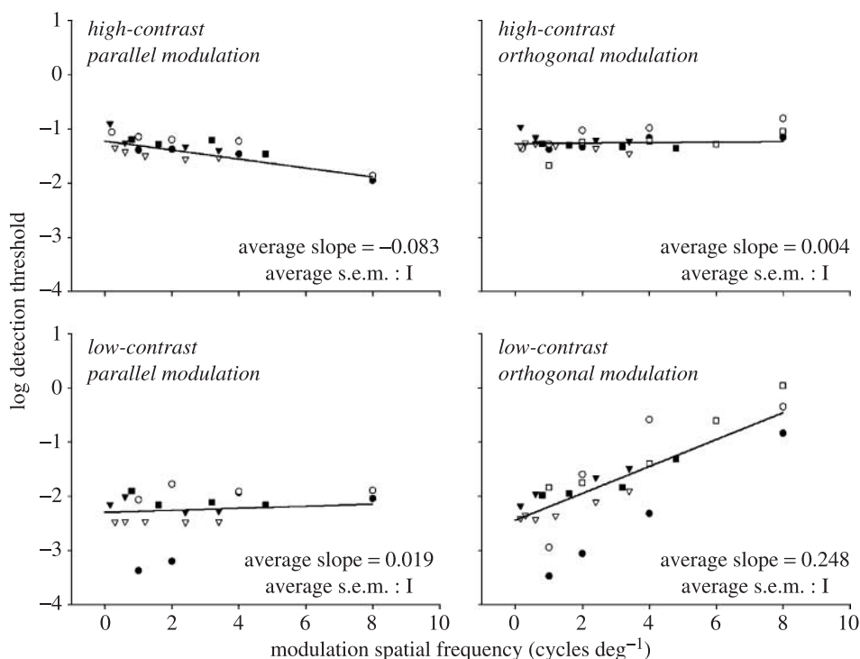
Figure 3. Data in the primary modulation detection task for six observers: T. M. (black circles), J. J. (white circles), M. W. (black triangles), T. L. (white triangles), I. F. (black squares) and I. M. (white squares). The y -axis represents log detection threshold, while the x -axis represents modulation spatial frequency in cycles \text{deg}^{-1} . ‘High contrast’ corresponds to a carrier contrast of 0.5 and ‘low contrast’ to a carrier contrast of 0.05. The carrier frequency for all conditions was 8.5 cycles \text{deg}^{-1} . The solid line corresponds to the average regression line for each set of data.
